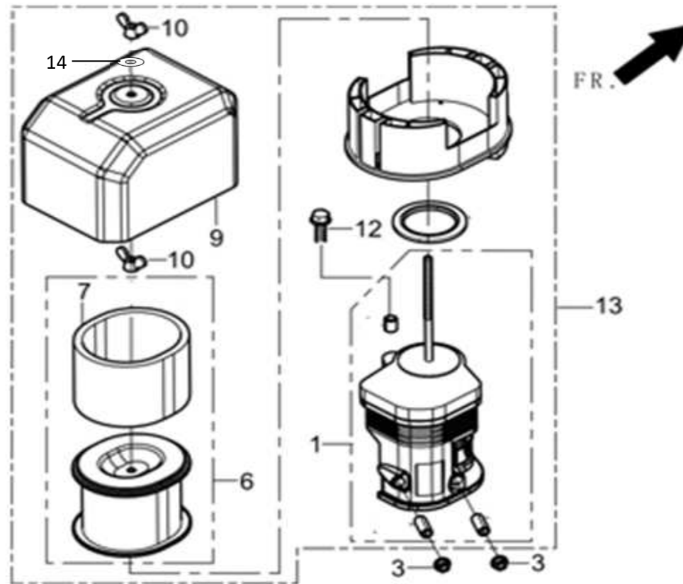
FIG.13 AIR CLEANER
