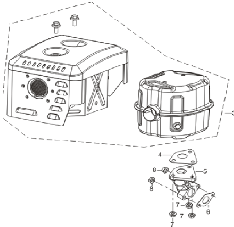
FIG.14 MUFFLER ASSEMBLY
