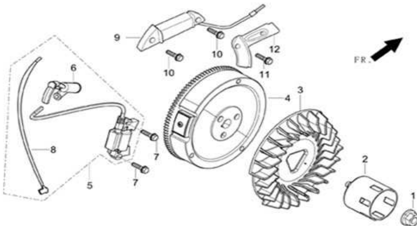
FIG.10 FLYWHEEL / IMPELLER / STARTER PULLEY / IGNITION COIL
