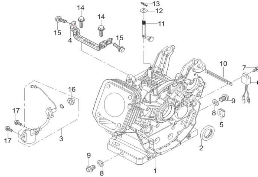
FIG.1 CRANKCASE/GOVERNOR GEAR ASSEMBLY
